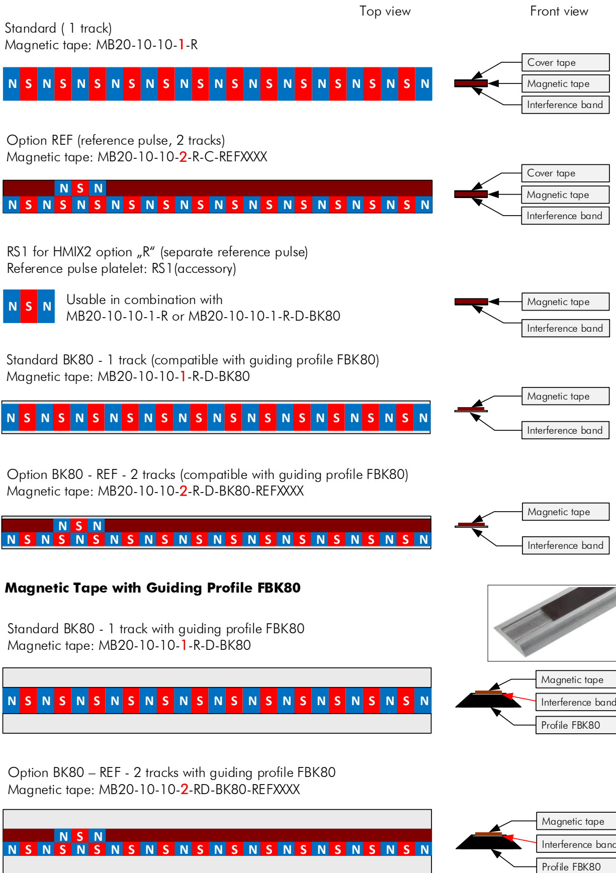
Figure 9: Magnetic Tape Variants
