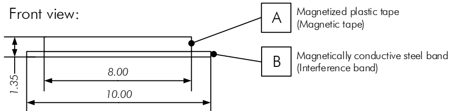
Figure 7: Magnetic Tape MB20-10-10-1(2)-R-D-BK80
