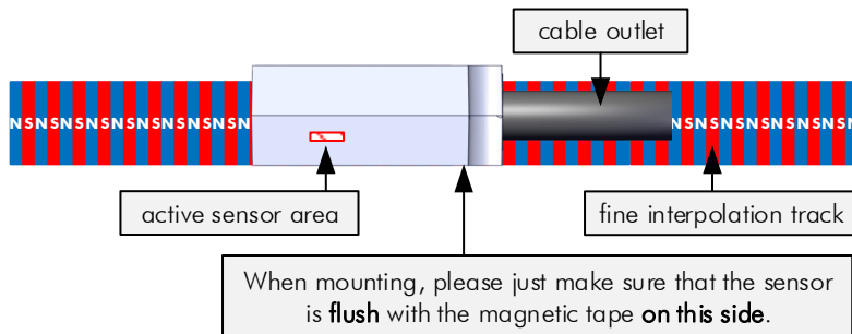
Figure 13: Alignment - HMIX2 (without Reference Pulse)
