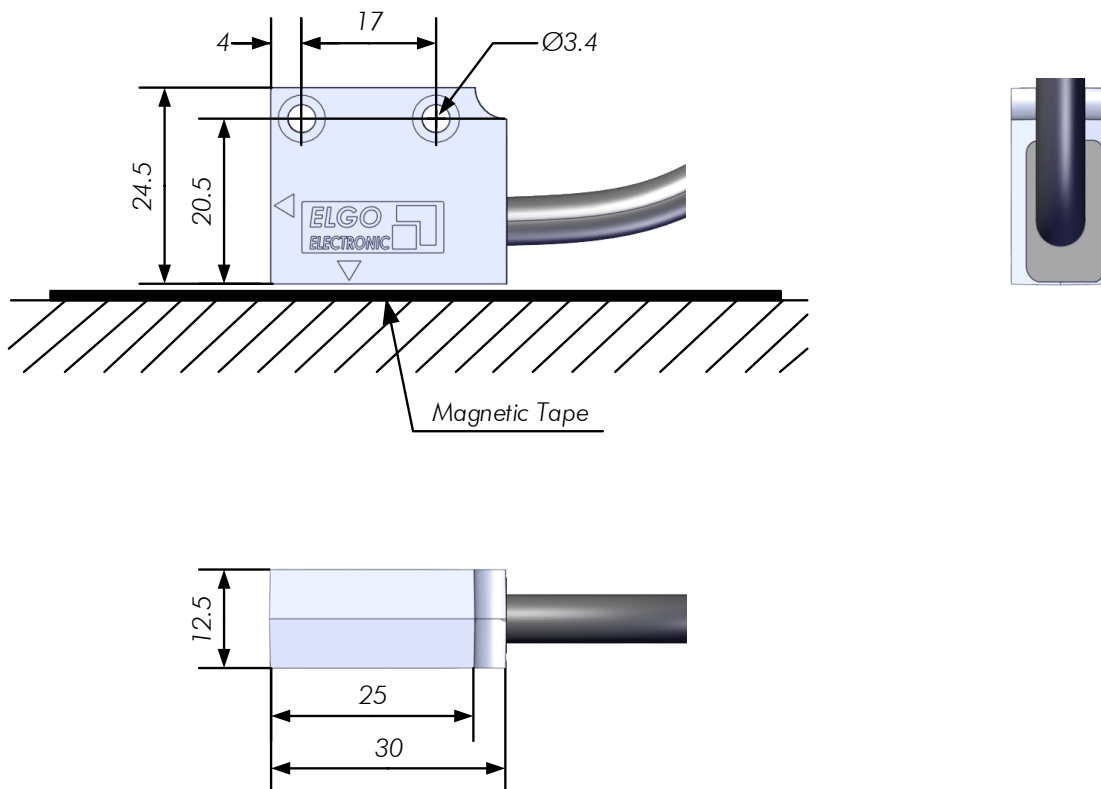
Figure 3: Dimensions Sensor
