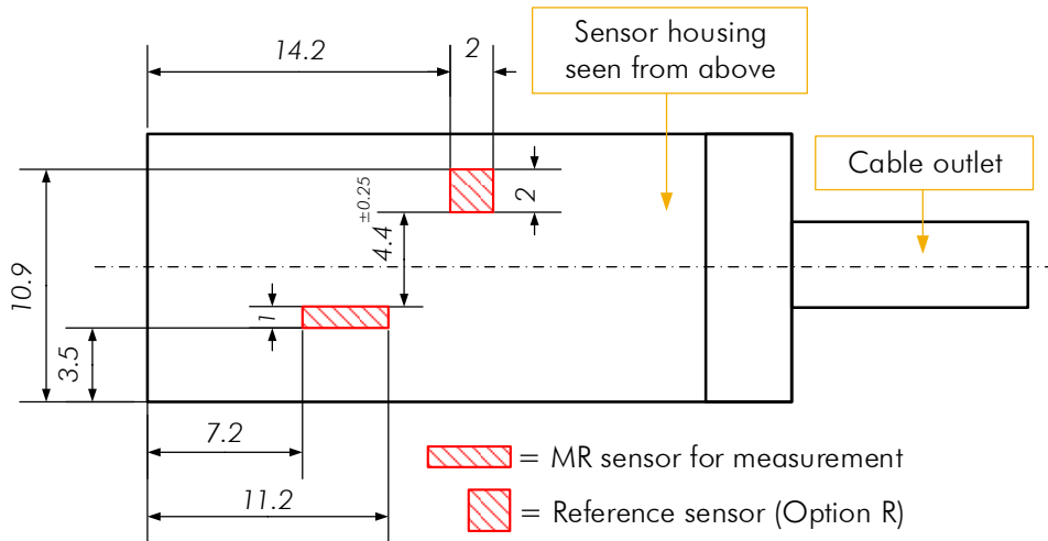
Figure 11: Active Sensor Areas
