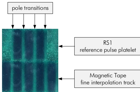
Figure 16: How to install the RS1 platelet
