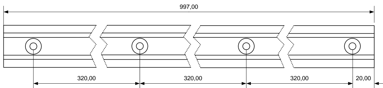
Figure 19: FBK80 Drawing
