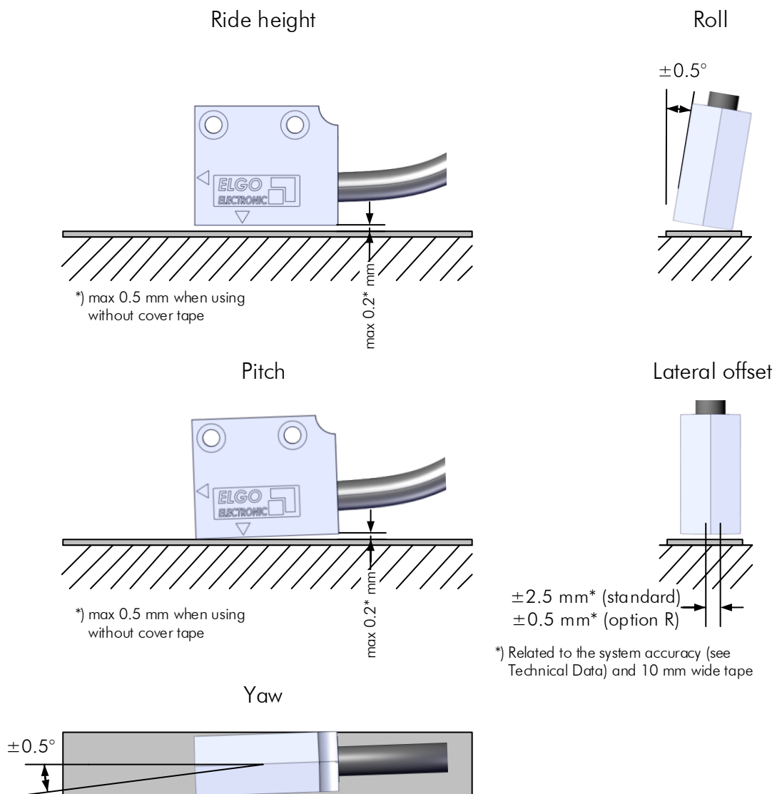
Figure 10: Tolerances
