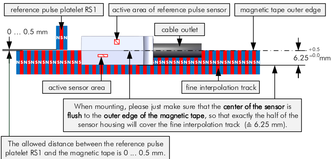
Figure 15: Alignment - Option R combined with "RS1" (Accessory)
