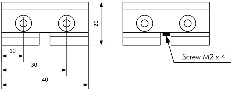
Figure 5: Dimensions AFBK 80
