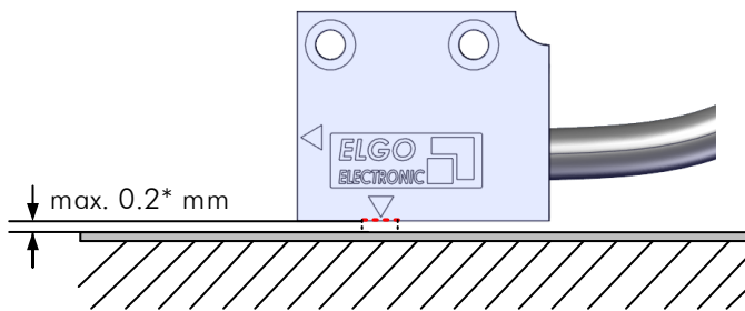
Figure 12: Mounting Distance - Sensor / Magnetic Tape
