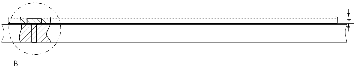
Figure 4: Dimensions FBK80
