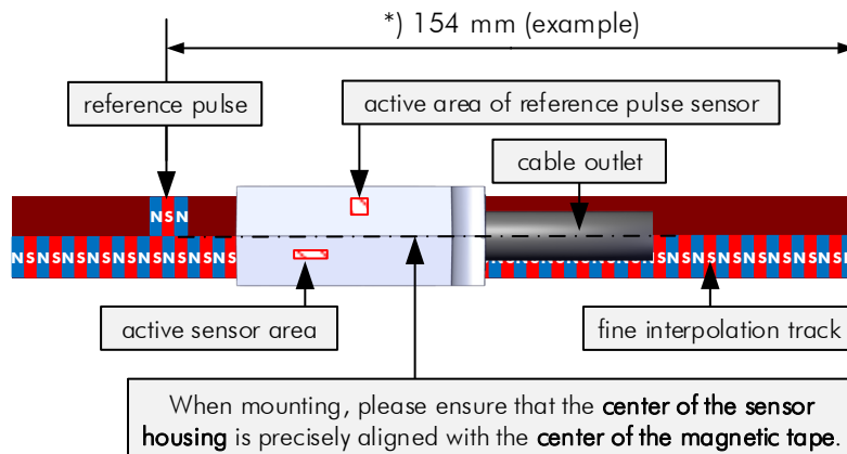
Figure 14: Alignment - Option R (Reference Pulse on Magnetic Tape Track)
