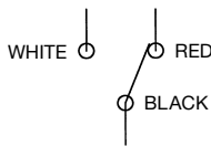
LEM6CASC SPDT CONTACT
