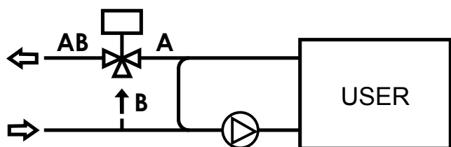
Mixing valve for constant flow to the user
