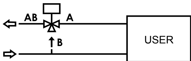
Mixing valve in diverting mode
