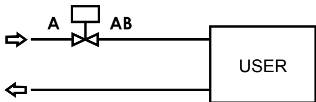
Valve with variable flow to the user
