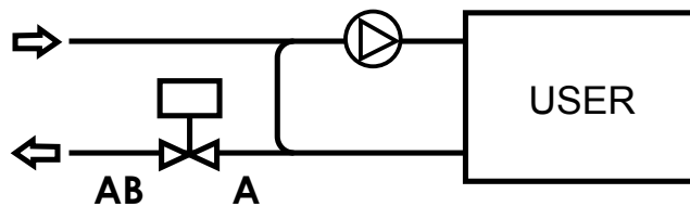
Valve with constant flow to the user
