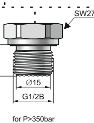
CG1/2 type G1/2" with flush diaphragm
