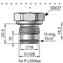
CG1/2 type G1/2" with flush diaphragm
